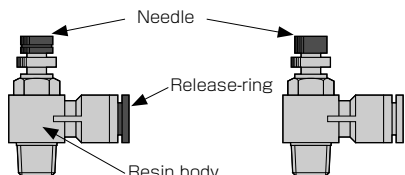
Throttle (Needle) Valve
