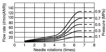
KJNC 6-02 8-02 10-02
