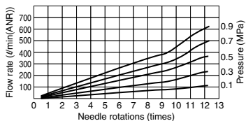
KJNC 10-04 12-04
