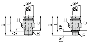
Taper pipe thread
